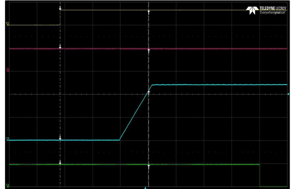
Figure 62: LCC600-48U-9P Turn-on delay via INH_EN Vin = 90Vac Load: I O = 12.5A (48V), I SB = 1.5A (5V) Ch 1: INH_EN Ch 2: V SB Ch 3: V O CH 4: G_DCOK_C
