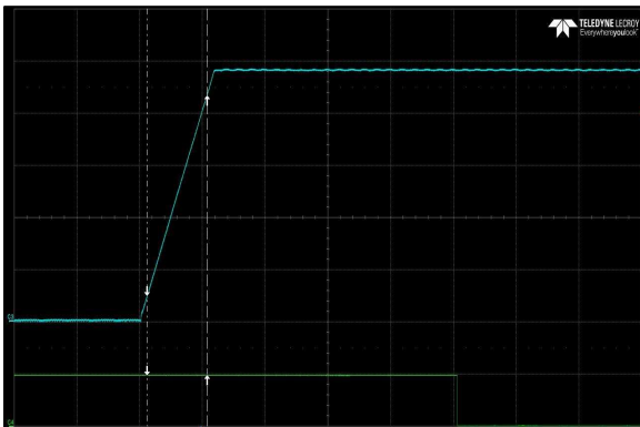
Figure 63: LCC600-48U-9P Hold-up Time Vin = 90Vac / 63Hz / 0° Load: I O = 12.5A (48V), I SB = 1.5A (5V) Ch 1: AC Mains Ch 2: V SB Ch 3: V O CH 4: G_DCOK_C
