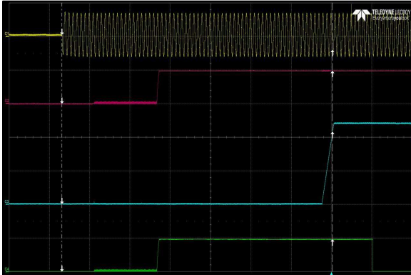
Figure 61: LCC600-48U-9P Turn-on delay via AC mains Vin = 90Vac Load: I O = 12.5A (48V), I SB = 1.5A (5V) Ch 1: AC Mains Ch 2: V SB Ch 3: V O CH 4: G_DCOK_C
