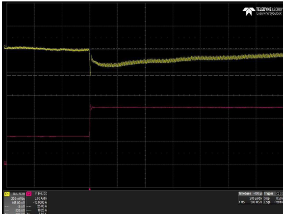
Figure 67: LCC600-48U-9P Transient Response - V_O Deviation 50% to 100% load change 1A/uS slew rate V_{in} = 230V_{ac} Ch 1: V_O Ch 2: I_O
