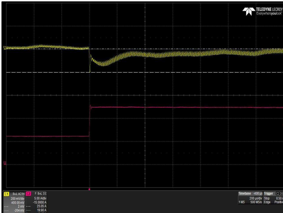
Figure 77: LCC600-48H-9P Transient Response - V_O Deviation 50% to 100% load change 1A/uS slew rate V_{in} = 277V_{ac} Ch 1: V_O Ch 2: I_O
