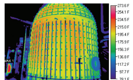
Gasifier thermal imaging screenshot
